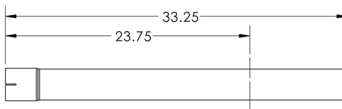
EXTENSION PIPE
